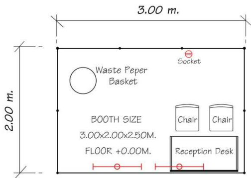
TOP VIEW SCALE 1:50
