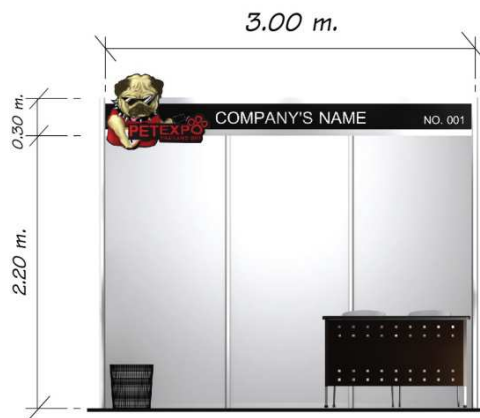
FRONT VIEW SCALE 1:50
