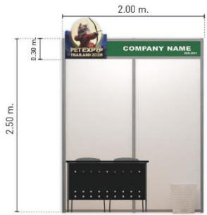
ELEVATION A SCALE 1:50
